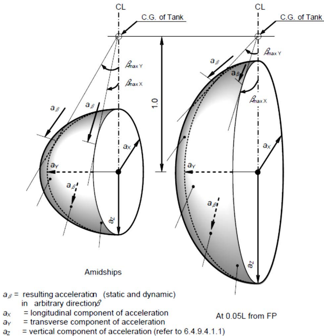
Figure 6.4.1 – Acceleration ellipsoid
